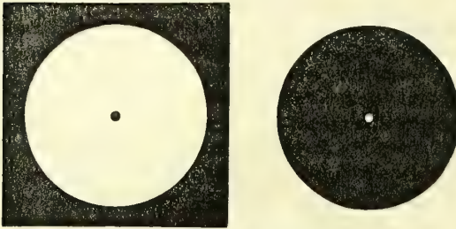
Apparent magnitude.
